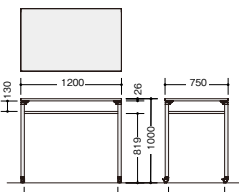
BTH1275C-□
