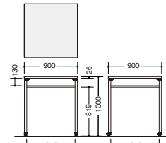
BTH0990C-□
