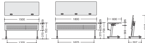
KUW1560SPT-□ KUW1860SPT-□
