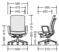
FEN513F-□
