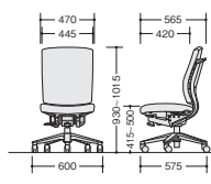
FEN512F-□
