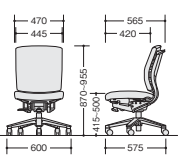
FEN510F-□
