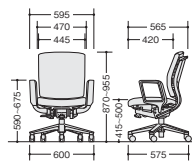
FEN511F-□
