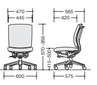
FEN510-□
