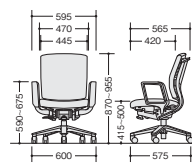
FEN511-□
